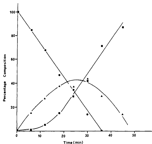
Figure 2. Time evolution of the MeDCA-sensitized photooxygenation of 2,3-di( p -methoxyphenyl)-1,4-dioxene ( 6a ) at 0 °C in acetone- d 6 . 1 H NMR spectroscopy was used to determine the concentration of 6a (●), the corresponding 1,2-dioxetane (▲), and the resultant cleavage product (■).
